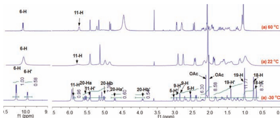
Scheme 1. ^1\text{H} NMR of Compound 3 (500 MHz Pyridine- d_5 )
