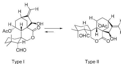
Figure 2. Two conformations of compound 3 .
