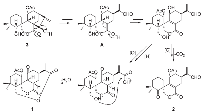
Scheme 2. Proposed Biogenetic Pathway of Compounds 1–3
