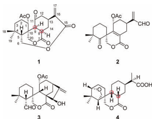
Figure 1. Structure of compounds 1–4 .
